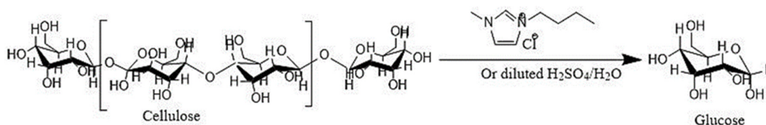
Figure 3. Cellulose hydrolysis to glucose
