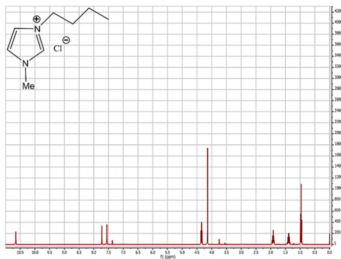
Figure 5. ^1\text{H} -NMR spectral of 1-butyl-3-methyl imidazolium chloride
